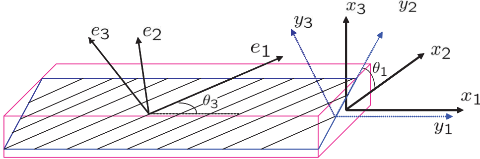
Figure 4: VABS layup convention
