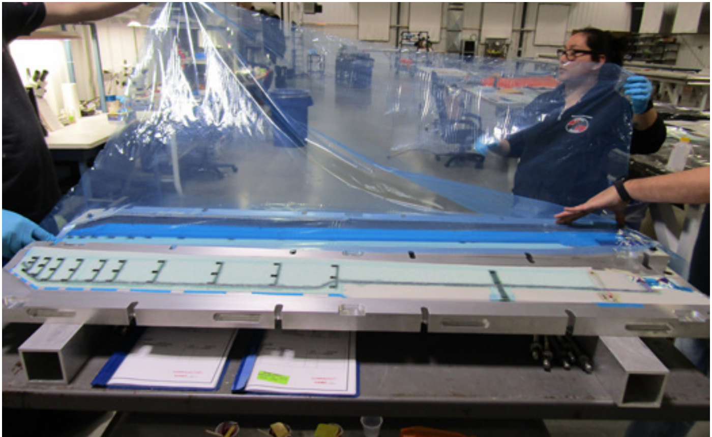
The HVAB blades use Rohacell foam spar cores and pre-cured instrumentation covers and leading-edge skins. ATI bonded the carbon-epoxy HVAB spars and instrumented fiberglass skins. (ATI photo)
